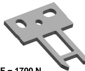
F = 1700 N LS-XG-ZBZ
