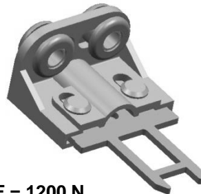
F = 1200 N LS-XNW-ZBZ
