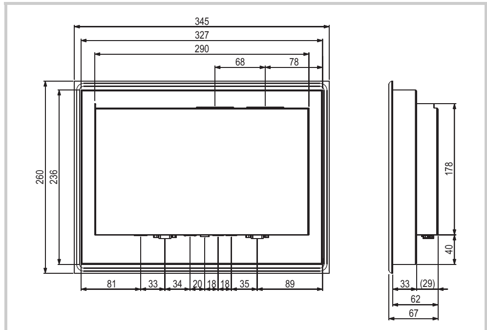
Fig. 30 Mechanical dimensions of the 10.4" devices in mm
