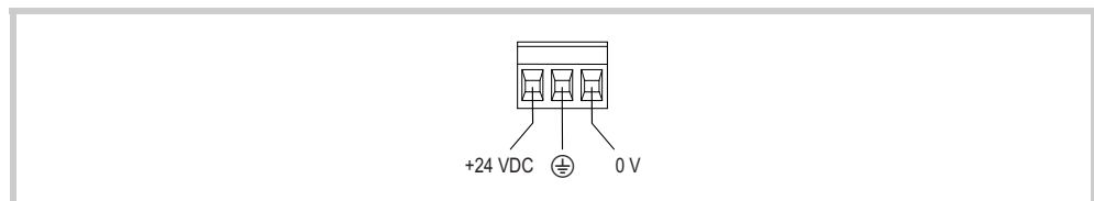
Fig. 12 Phoenix Contact MSTB 2.5/3-ST-5.08 connector (view from the wiring side)
