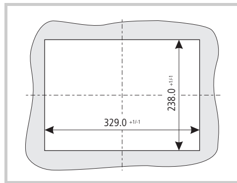
Fig. 19 Mounting cutout for 10.4" devices
