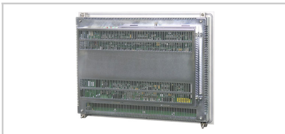
Fig. 24 10.4" and 12.1" devices with four retaining brackets (do not meet IP65 requirements)
