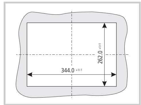
Fig. 20 Mounting cutout for 12.1" devices
