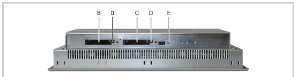
Fig. 5 Operating elements on the service side (CF slot cover removed)
