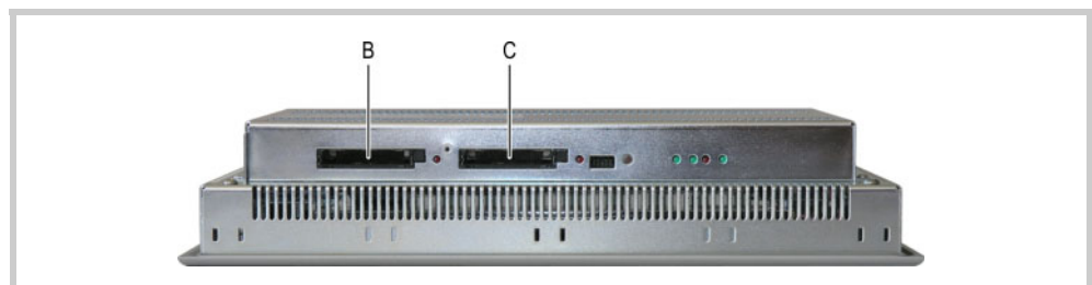
Fig. 29 Service side of the device (CF slot cover removed)
