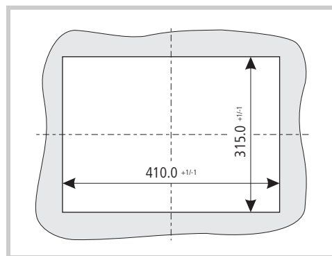
Fig. 21 Mounting cutout for 15" devices
