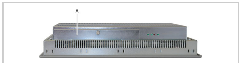
Fig. 28 Service side of the device (CF slot cover fitted)
