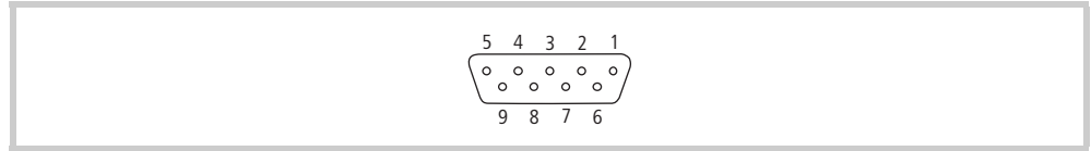
Fig. 17 Profibus interface (9-pin, D-Sub, female, UNC)
