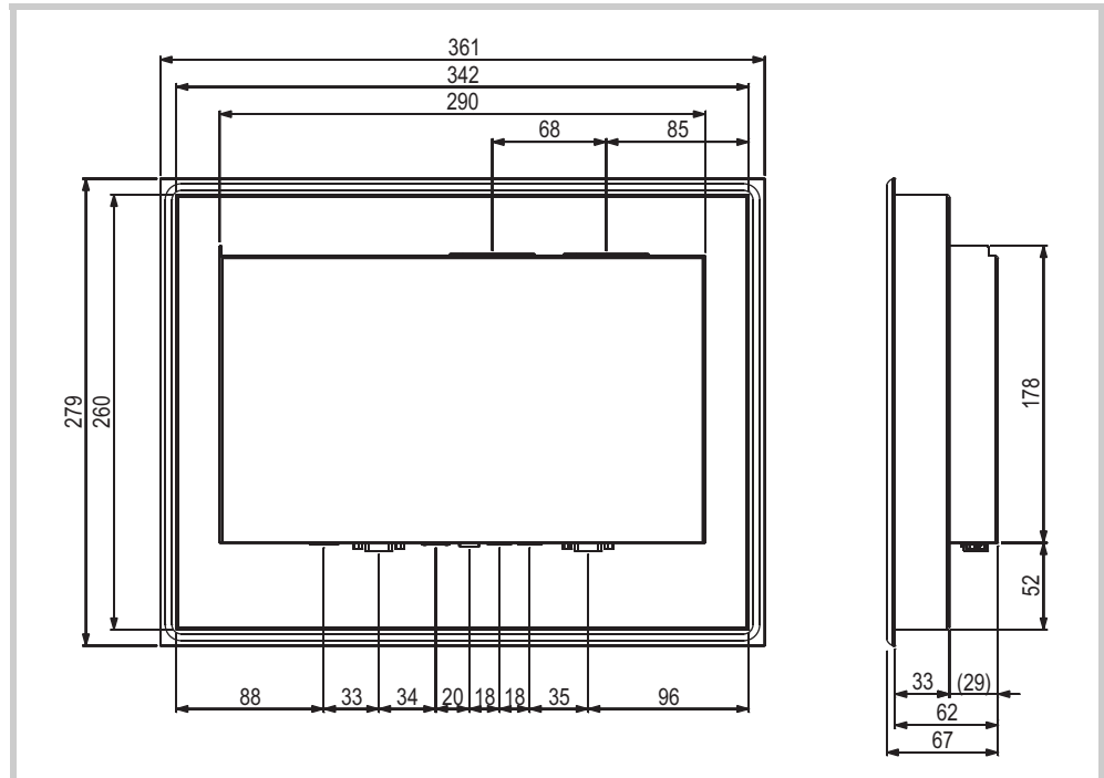
Fig. 31 Mechanical dimensions of the 12.1" devices in mm
